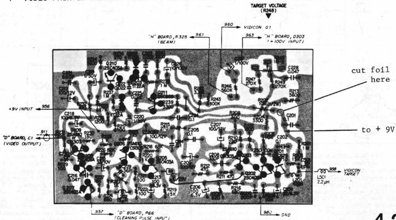
"P" VIDEO PRINTED CIRCUIT BOARD - CONDUCTOR SIDE
